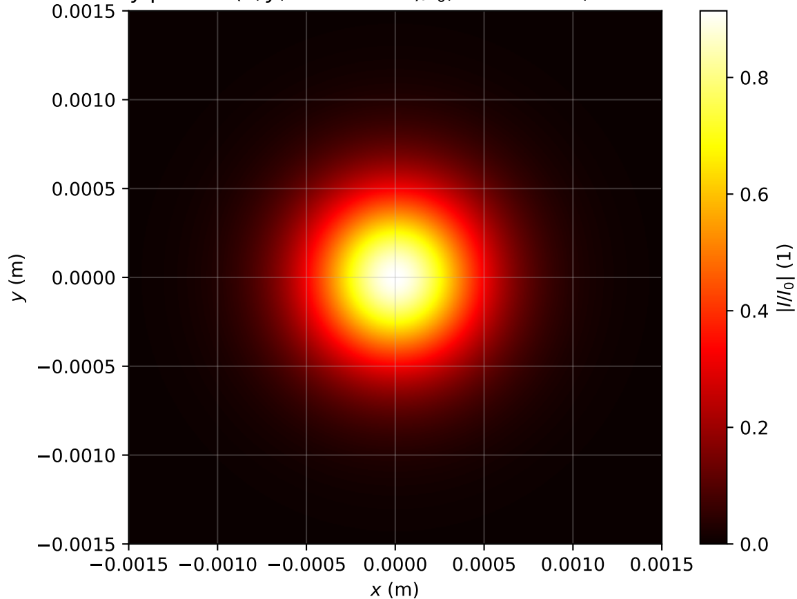
Intensity profile I(x, y, z = 1.672m)/I_0 , Pin=0.5Pcr, artificial time
